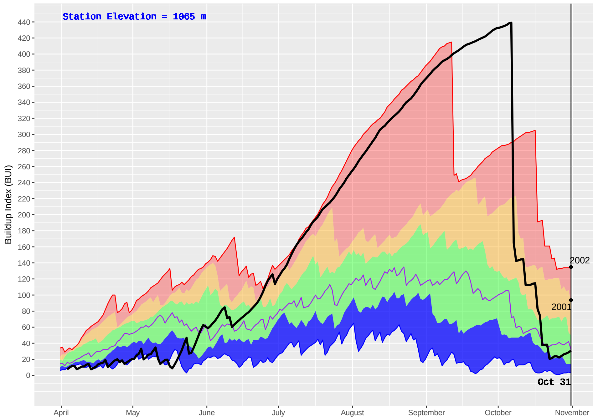
ASPEN GROVE (302) : Historical (1998–2016) and Current (2017) Noon Buildup Index (BUI)
